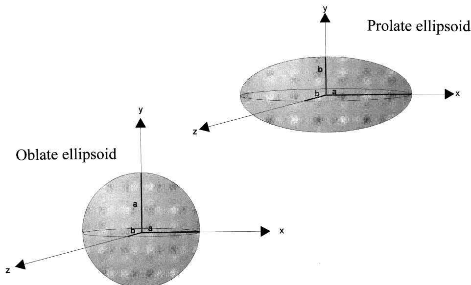
Fig. 2 Ellipsoids of revolution. A prolate ellipsoid has semi-axes ( a, b, b ). An oblate ellipsoid has semi-axes ( a, a, b ). The shapes of both are represented by a single axial ratio ( a/b ), with a \geq b
