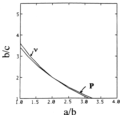
Fig. 5 Triaxial ( a/b , b/c ) plot showing that a single value of a Universal shape function corresponds to a range (specified by a line) of possible values of ( a/b , b/c ). Two examples shown: \nu=3.8016 and P=1.1302
