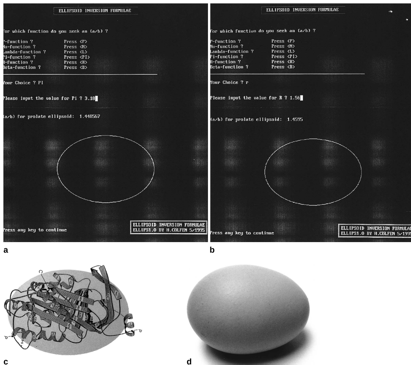
Fig. 3 ELLIPS1 output screens for the determination of the axial ratio ( a/b ) for ovalbumin (egg albumin) using the Universal shape functions (a) \Pi or (b) R . (c) Prolate ellipsoid of a/b=1.5 drawn by the WINDOWS based CORELDRAW enclosing the crystal structure line-drawing of Stein et al. (1991). (d) A standard egg of a/b \sim 1.5
