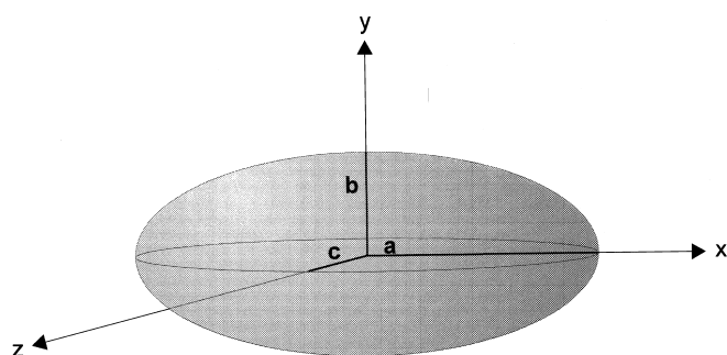
Fig. 1 The general ellipsoid. It has three semi-axes ( a \geq b \geq c ) and its shape is represented by two axial ratios ( a/b, b/c )
