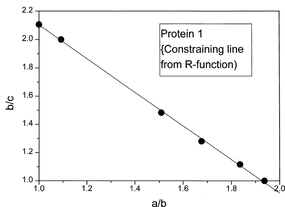
Fig. 9 ELLIPS4 constraining data extraction. The user takes his determined value of R or other suitable constraining function ( \Pi , G , \Delta etc.) and plots the line of corresponding values of (a/b, b/c) using ELLIPS3 (ELLIPS3 gives 2 lines which allow for experimental error, both of which can be used in successive runs using ELLIPS4. It also plots 2 lines for a 2nd function which should be entered = 0). The user then reads off 6 (a/b, b/c) coordinates from this line which can be either entered as a 2nd data file into ELLIPS4, or instead entered at run-time
