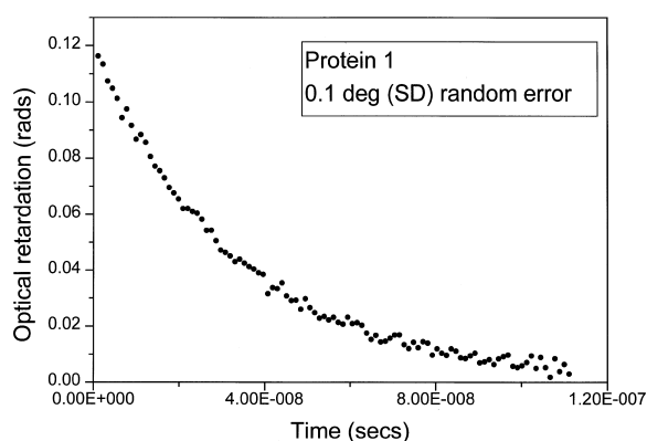
Fig. 8 Electro-optic decay (expressed as the decay of optical retardation with time, t [s]). Synthetic data shown corresponding to a protein of true ( a/b , b/c ) = (1.5, 1.5) {“Protein 1” of Harding and Rowe 1983}. The electro-optic data is fed in as a date-file into ELLIPS4
